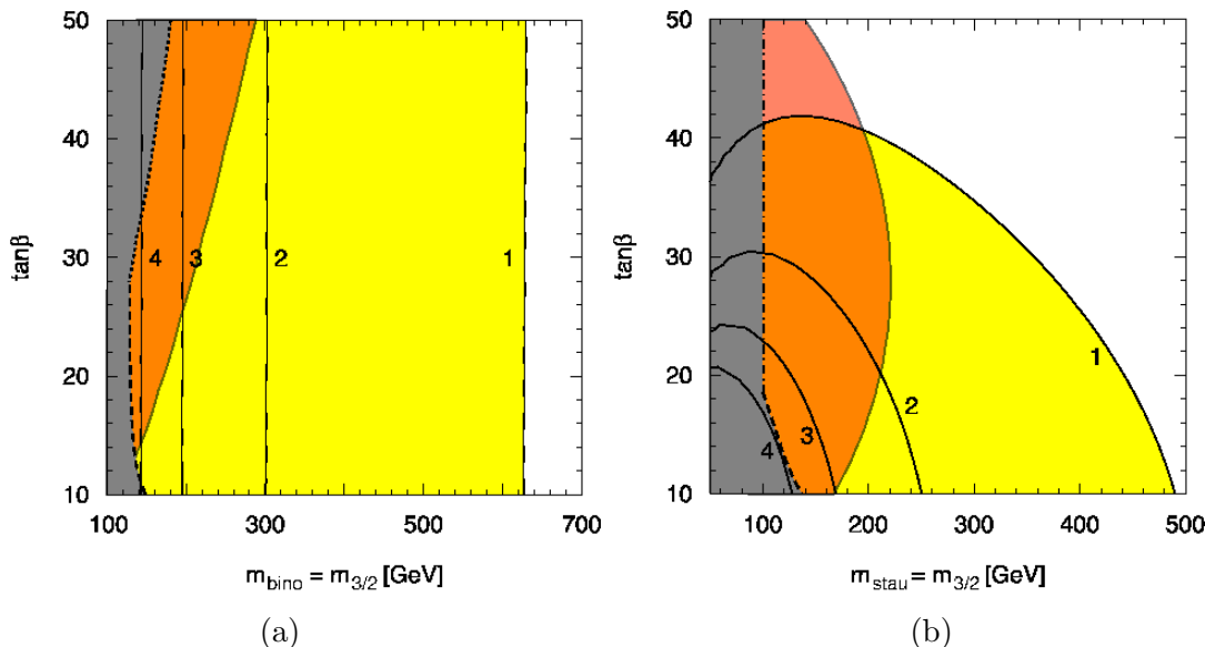
Figure 1: Contours of constant reheating temperature, T_R = (1 - 4) \times 10^9 GeV, with \Omega_{3/2} = \Omega_{\text{DM}} (solid lines) (cf. eq. (3.6)). The panels (a) and (b) correspond to the GUT boundary conditions (A) and (B) with bino-like NLSP and stau NLSP, respectively. The choice m_{3/2} = m_{\text{NLSP}} maximizes the reheating temperature. The gray region is excluded by constraints from low-energy experiments: the lower \tan \beta part (left of the dashed line) does not satisfy the LEP Higgs mass bound; the higher \tan \beta part in (a) (left of the dotted line) is ruled out by \text{Br}(B_d \rightarrow X_s \gamma) ; the higher \tan \beta part in (b) (left of the dot-dashed line) does not satisfy the lower mass bound on charged particles from LEP. Thermal leptogenesis is possible in the yellow and orange regions; the orange region is favored by the muon g - 2 anomaly at the 2\sigma level.
